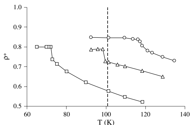
Figure 7. Effect of the wall/fluid interaction on the density of Lennard-Jones methane confined in a smooth slit-like pore with H = 7.5\sigma ( \sigma being the diameter of methane). (O) ‘Graphite wall’ corresponds to a strongly attractive wall, and (□) ‘hard wall’ corresponds to a purely repulsive wall. (△) ‘Methane wall’ corresponds to a system with wall/fluid interaction similar to the fluid/fluid interaction. The straight vertical line indicates the bulk freezing temperature. Adapted from Miyahara and Gubbins [233].
